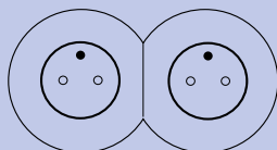
Double horizontal porcelain cover plate dimensions 154x83x7mm
